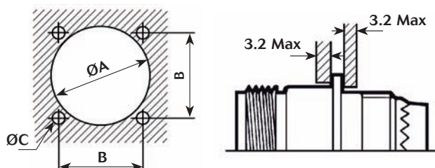
Type 0 square flange receptacle
