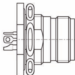
Type 7: Jam nut receptacle
